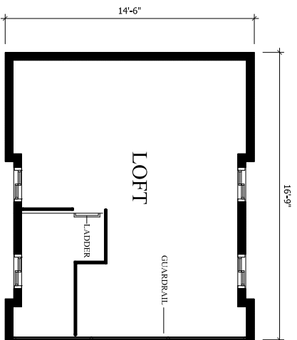
LOFT PLAN 222 SQ FT
